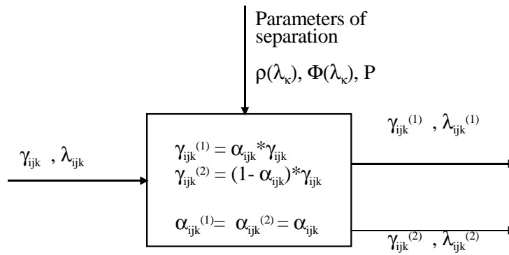
Fig.1 The model of a technological separation process
